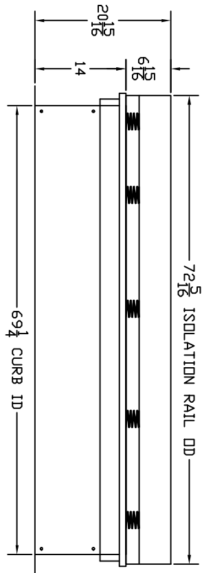
FRONT VIEW
