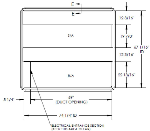
EXISTING CURB
